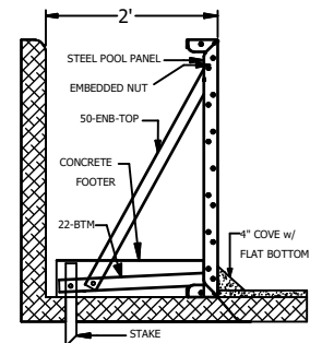
OPTION 3 (REPLACE x2 48" PANELS)
