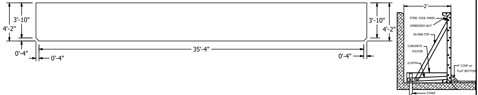
ST-1020ENB-52 (SIDE PROFILE)
